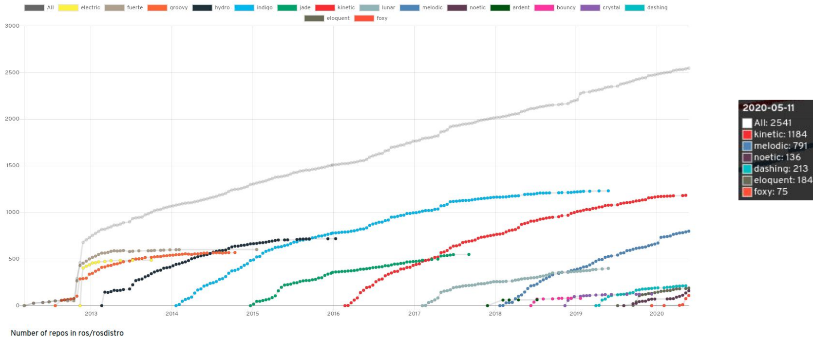
Number of Repositories in rosdistro
