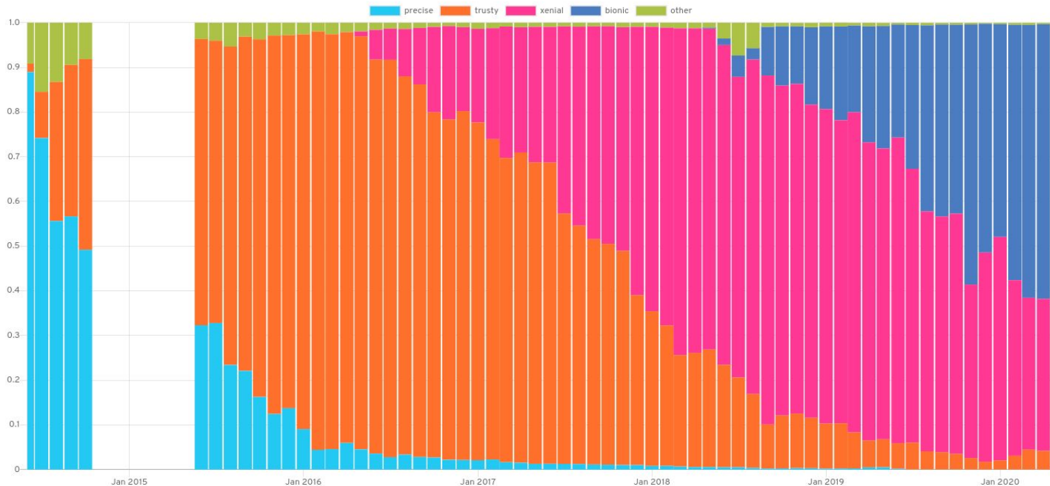
Linux Distro Usage by packages.ros.org traffic
