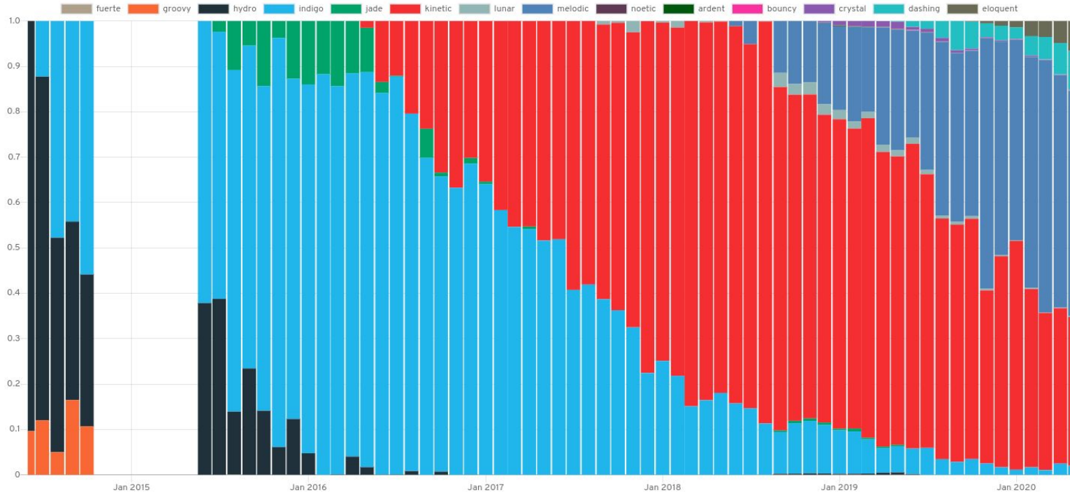
ROS Distro Usage by packages.ros.org traffic
